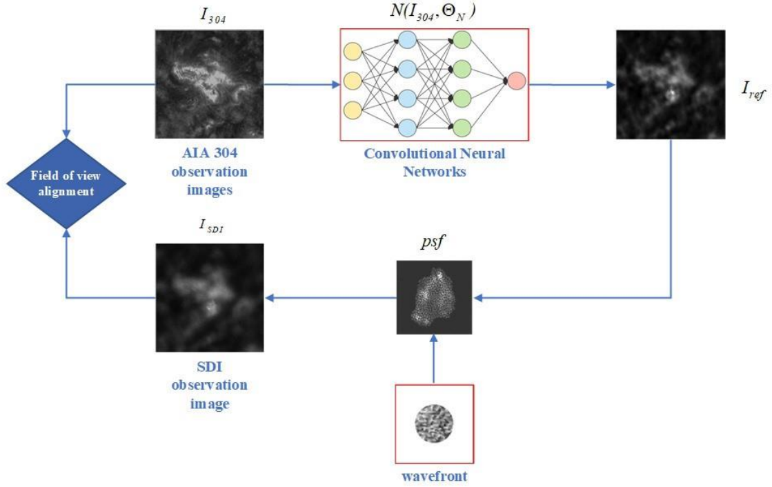
Fig.3: Flow chart of instrumental psf estimating process.
