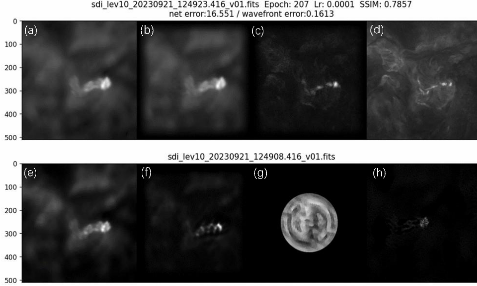
Fig.4: Intermediate Results of SPIBOA Training Process. (a) SDI observational image for training; (b) I_{ref} \otimes psf ; (c) I_{ref} ; (d) I_{304} ; (e) SDI observational image for testing; (f) deconvolution of the test image with the obtained psf ; (g) wavefront generated by SPIBOA; (h) psf obtained from the wavefront using Equation (3).
