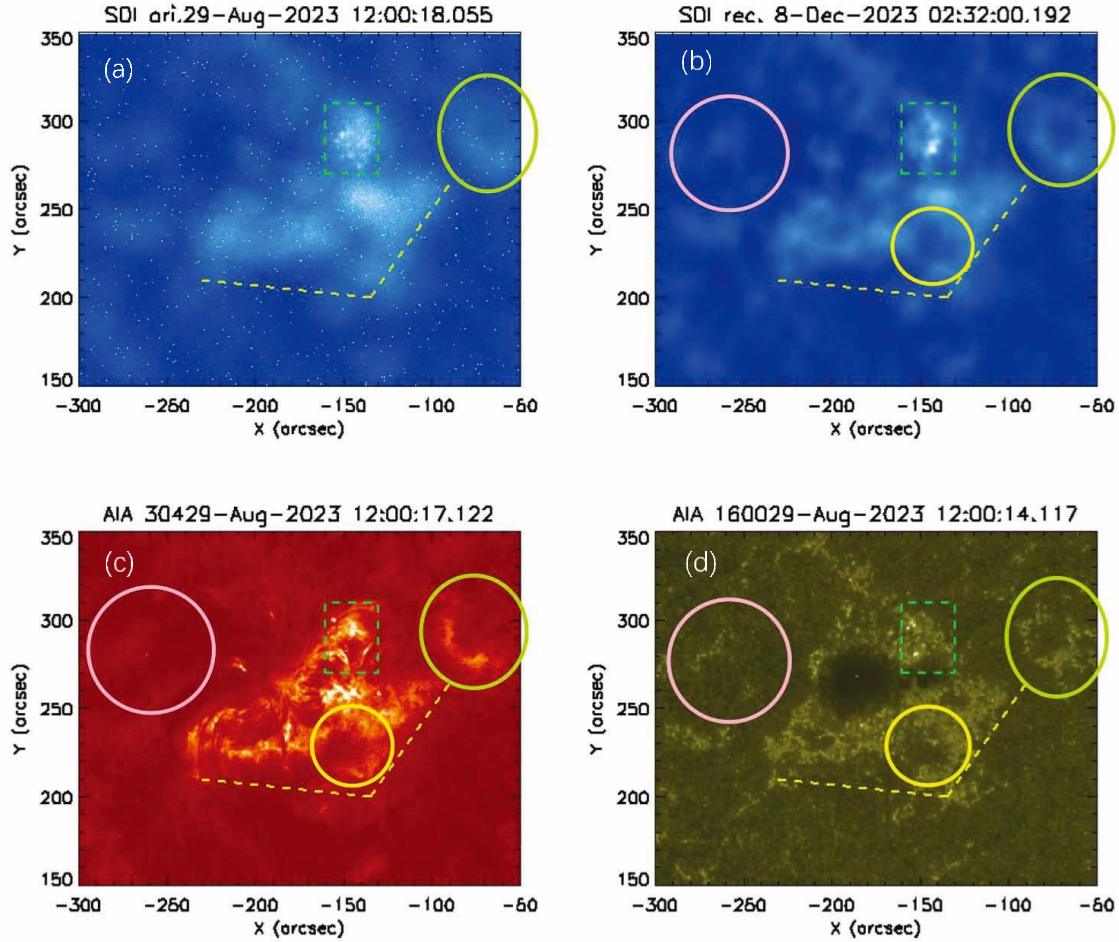
Fig.9: Comparison of (a) original and (b) reconstructed SDI images with (c) AIA 304 A and (d) 1600° A° images.
