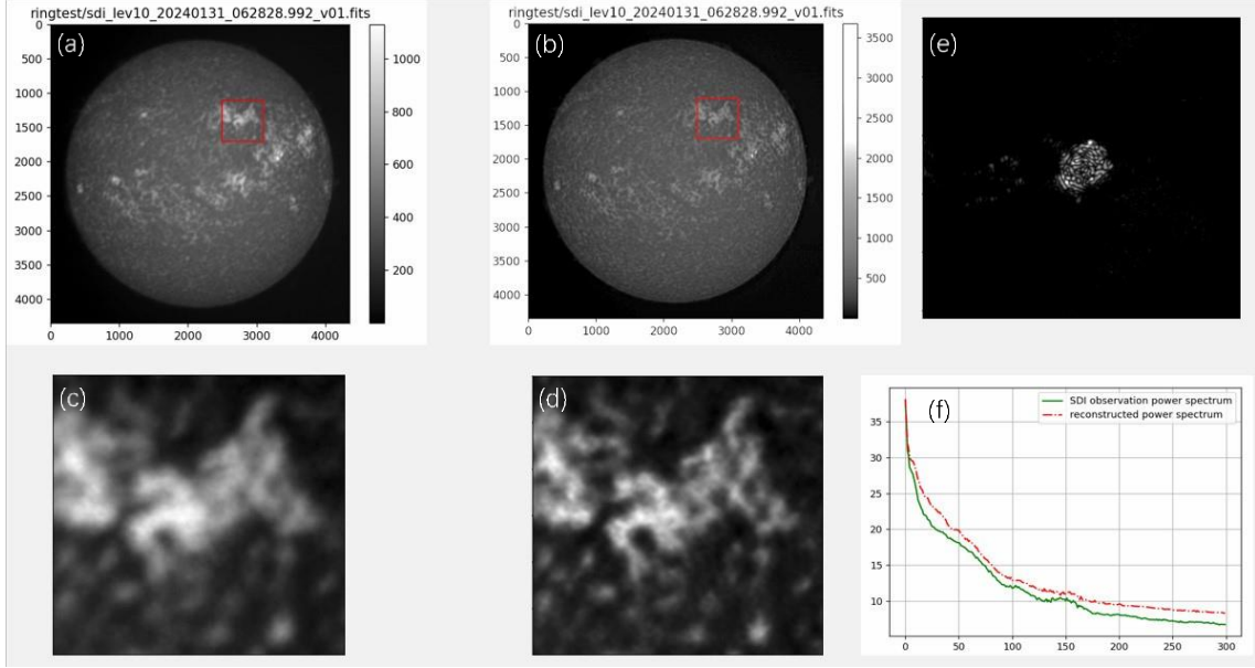
Fig.5: Deconvolution with PSF obtained by SPIBOA and power spectrum. (a) SDI observational image; (b) deconvolution image; images in panels (c) and (d) correspond to the sub-region denoted by the red box in panels (a) and (b), respectively; (e) The psf obtained from SPIBOA; (f) The power spectral density profiles of image in panel (c) (green) and panel (d) (red); the abscissa in (f) stands for normalized frequency while the ordinate for power density.
