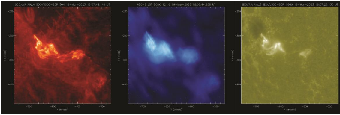
Fig.2: Comparison of AIA 304 Å (left), SDI (middle) and AIA 1600 Å (right) images at 18:07 UT on 2023 o March 19.
