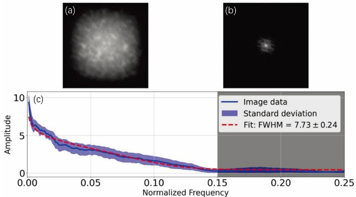
Fig.8: Same as Figure 7 but for the corresponding reconstructed image.
