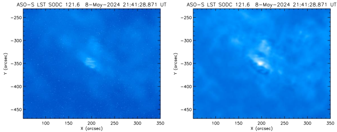
Fig.10: Cutout of observed (left panel) and reconstructed (right panel) SDI image of 2024 May 8. The reconstructed image shows the ring artifacts around the brightening area.
