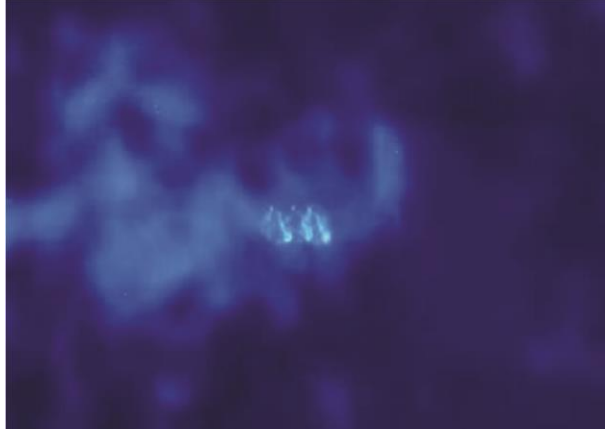
Fig.1: A cutout of SDI sample image showing ‘horseshoe’ brightenings.
