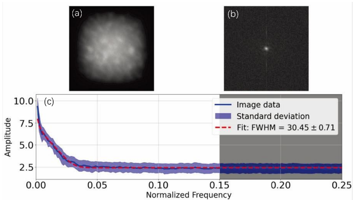
Fig.7: Spatial resolution estimate with SIRAF of SDI image obtained on 2024 May 8. (a) selected region of SDI image filtered using a Hanning window; (b) FFT transformed image in the frequency domain; (c) results of the fitting of the PSF function: its abscissa and ordinate indicate the normalized frequency (in unit length of the reciprocal of image size) and amplitude, respectively. The blue line represents the amplitude spectrum, and the red dashed line represents the fitting curve.
